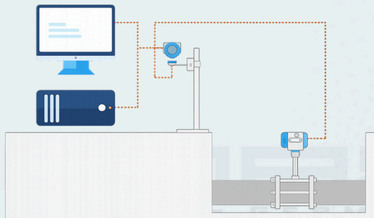
REMOTE VORTEX FLOWMETER INSTALLATION DIAGRAM
